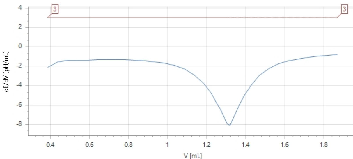
Measured Values Scope 1/1, Sample 24/30
