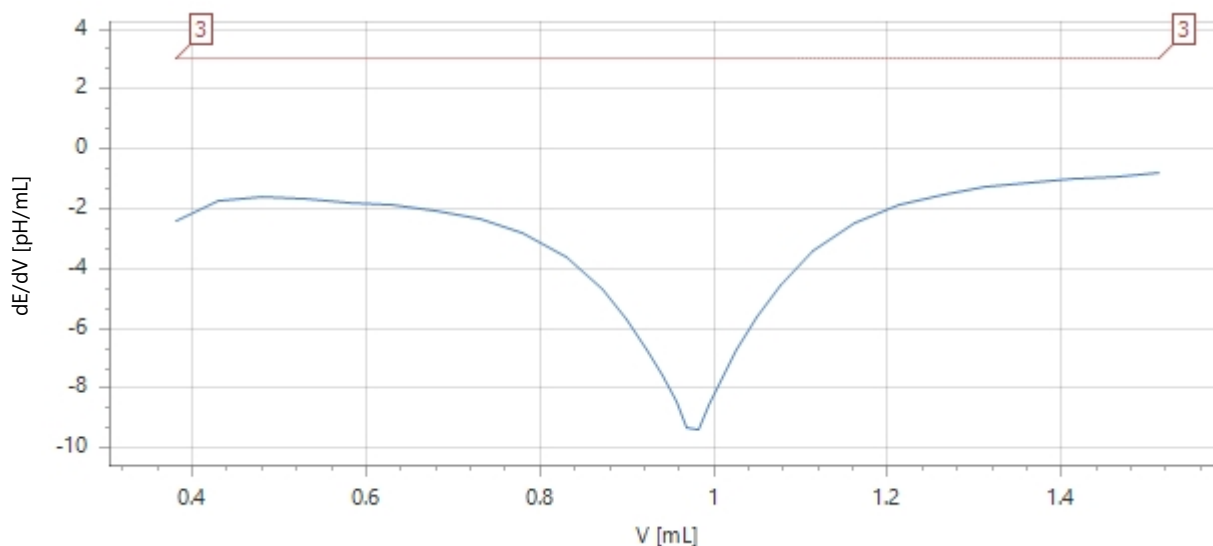
Measured Values Scope 1/1, Sample 11/30
