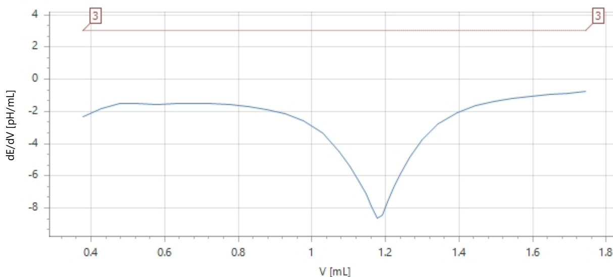
Measured Values Scope 1/1, Sample 2/30
