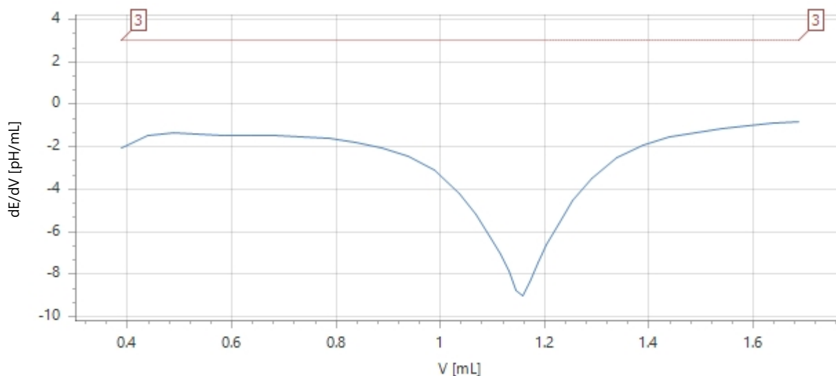
Measured Values Scope 1/1, Sample 15/30
